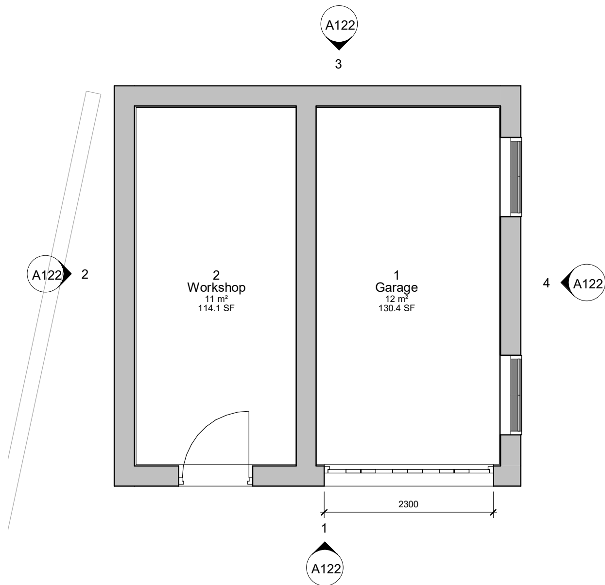
Proposed Ground Floor 1 : 50
