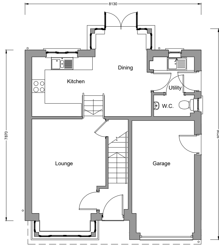
Ground/Lower Ground Floor Plan
