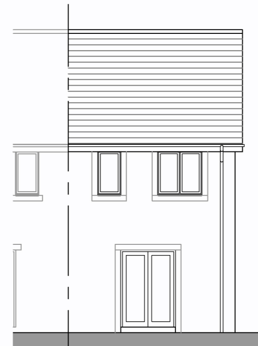
REAR ELEVATION
