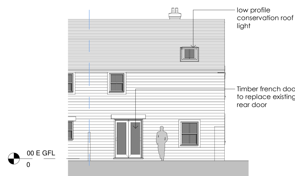
3 Proposed Rear (west) Elevation 1 : 100
