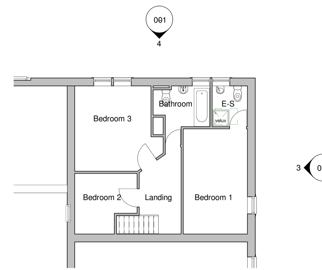
10 Proposed First Floor Plan 1 : 100
