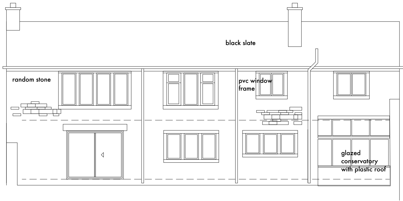
3 Front Elevation 1:100
