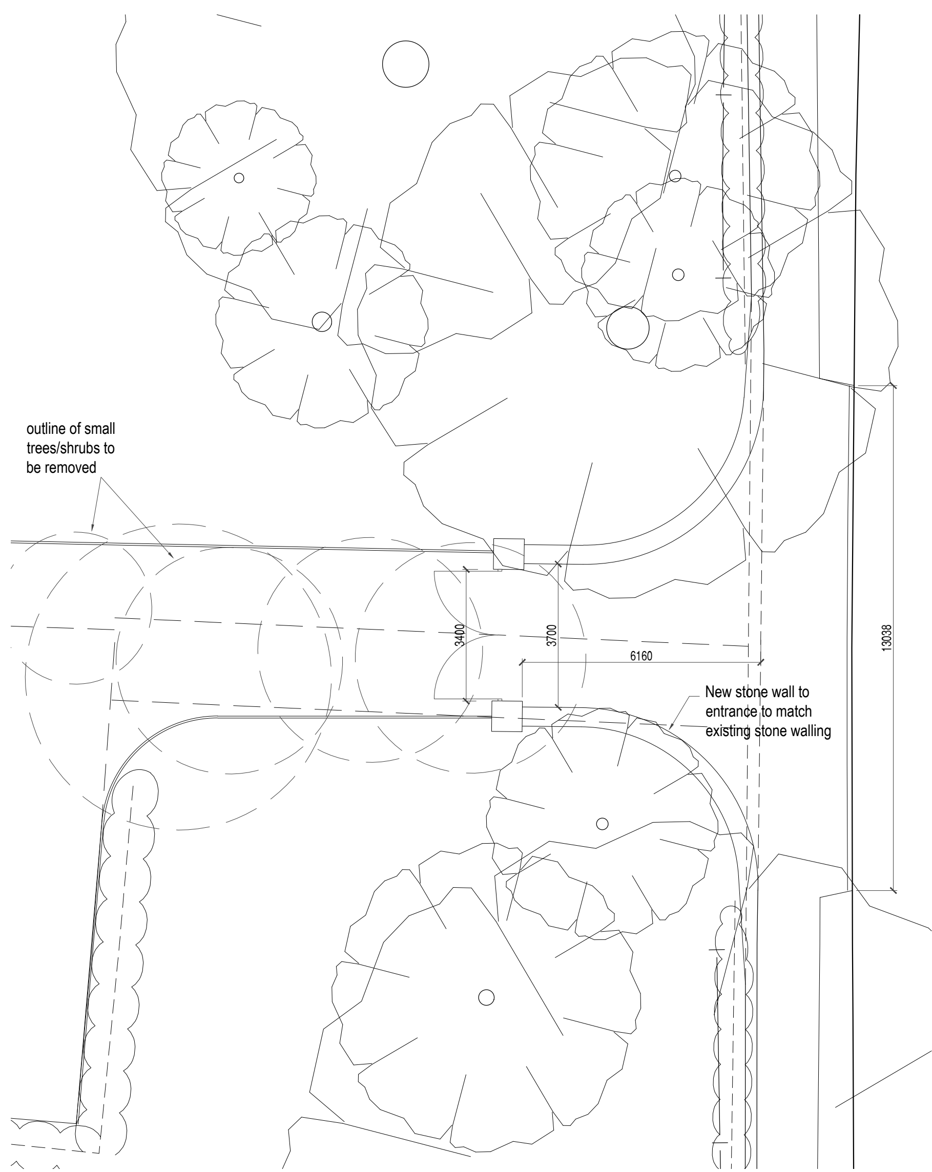
ENLARGED SITE ENTRANCE DETAIL 1:50
