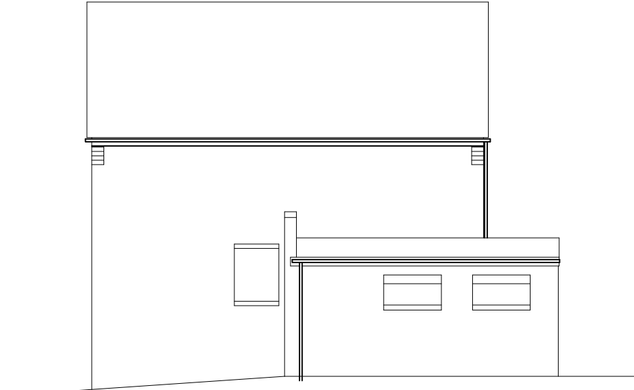
Existing Gable Elevation
