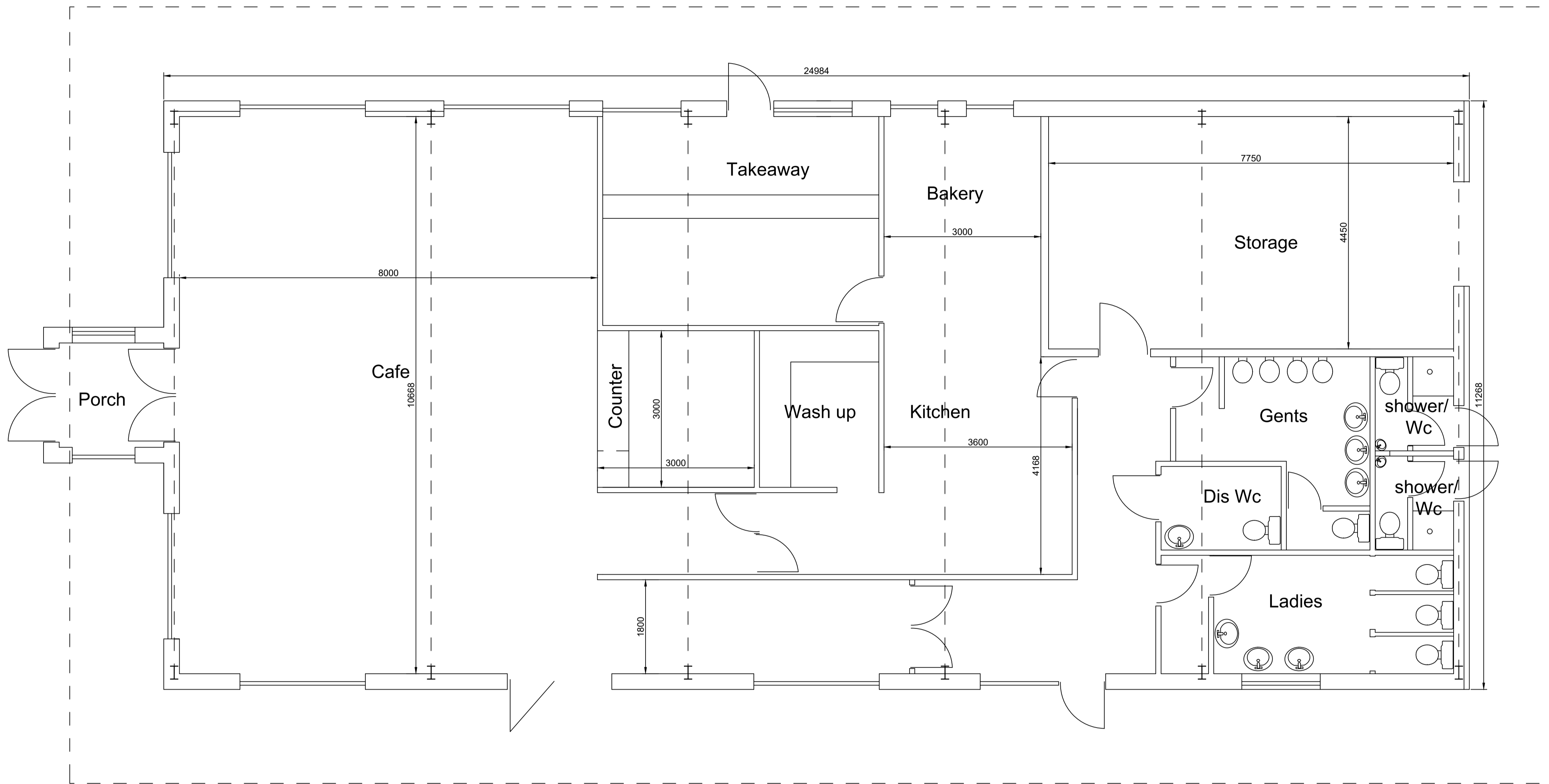
PROPOSED CAFE BUILDING
