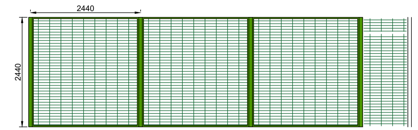
Fence To Play Area perimeter Typical Detail 1:50
