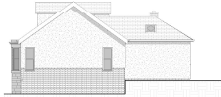
5 PROPOSED EAST 1 : 100
