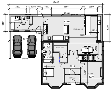
1 PROPOSED GROUND FLOOR 1 : 100
