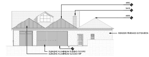
4 PROPOSED NORTH 1 : 100
