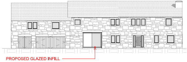
1 PROPOSED GLAZED INFILL 1 : 200
