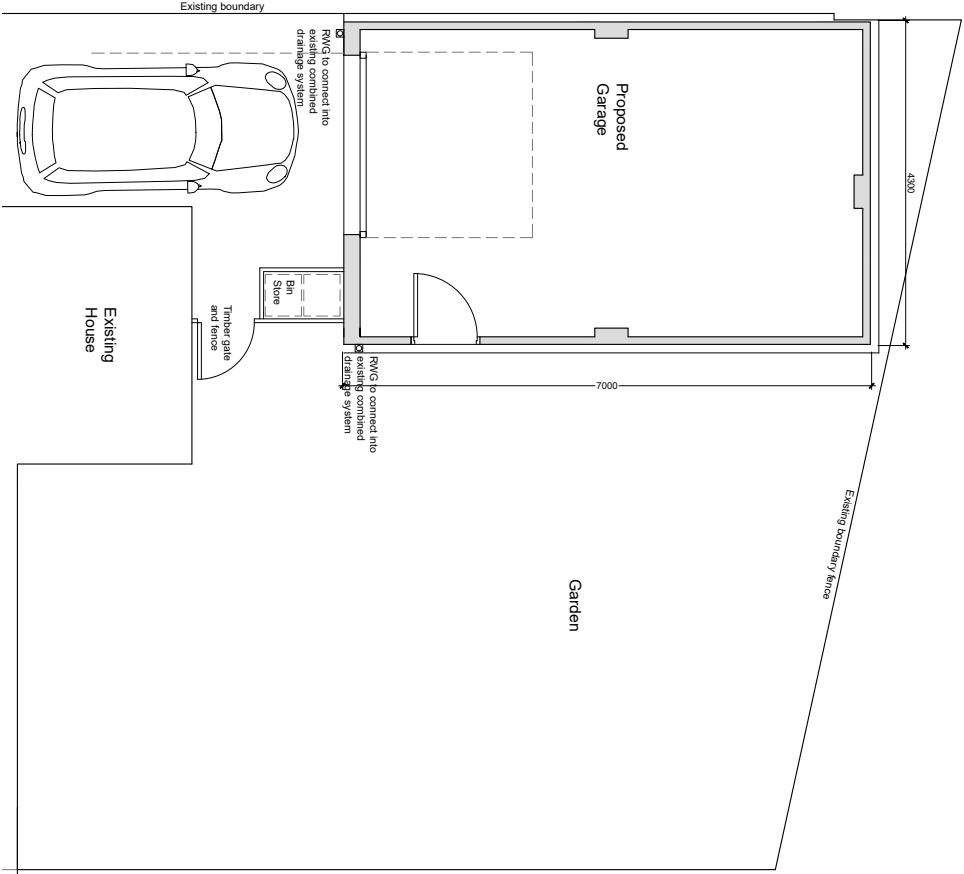
Floor/Site Plan 1:50 Scale
