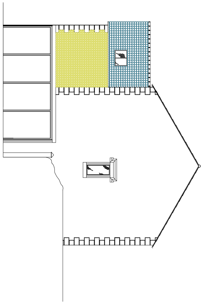
South Elevation
