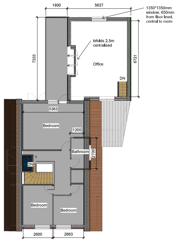
2 1st floor 1 : 100
