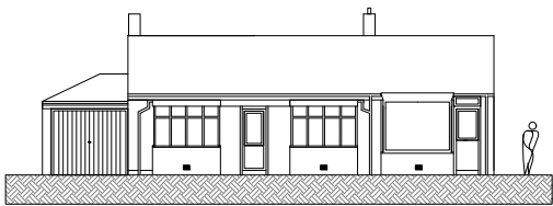
EXISTING SOUTH EAST ELEVATION
