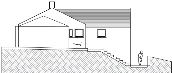
PROPOSED NORTH EAST ELEVATION
