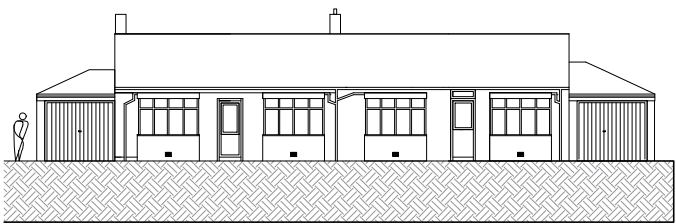
PROPOSED SOUTH EAST ELEVATION
