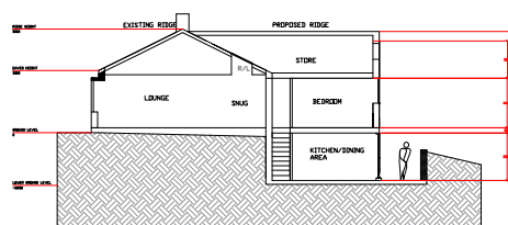
PROPOSED SECTION
