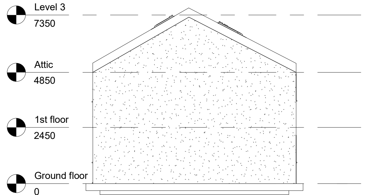
2 Party wall side 1 : 100
