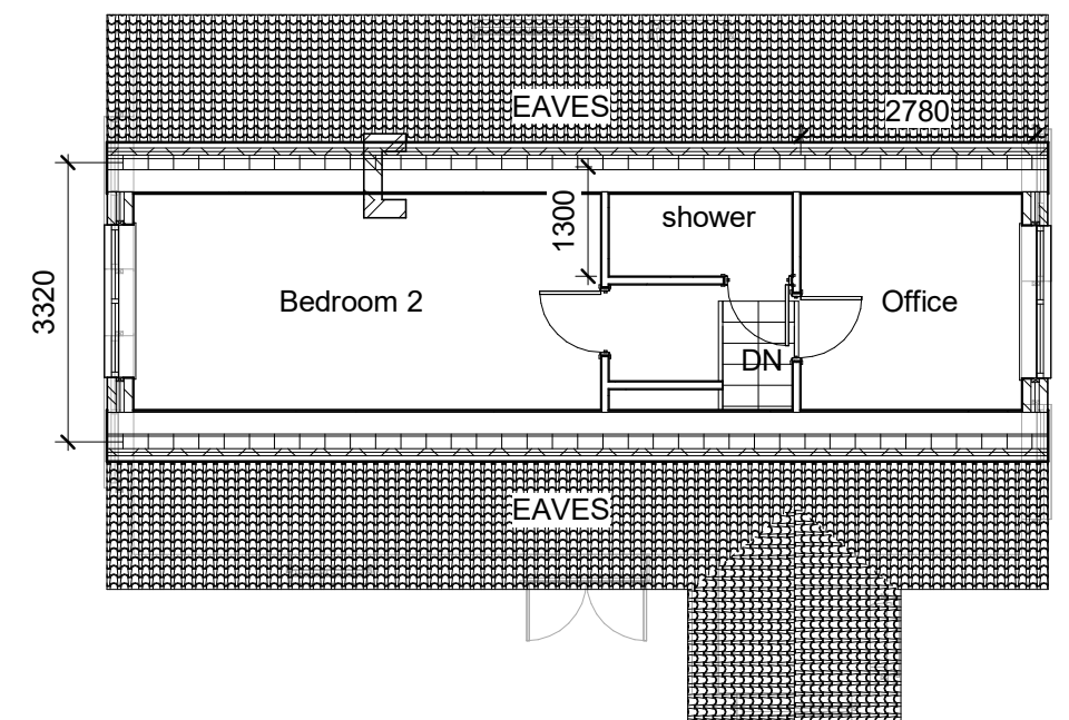
2 1st Floor 1 : 100
