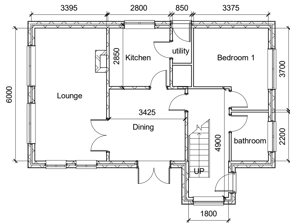
1 Ground floor 1 : 100
