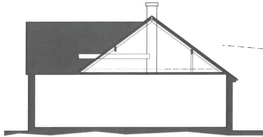
Typical Section A
