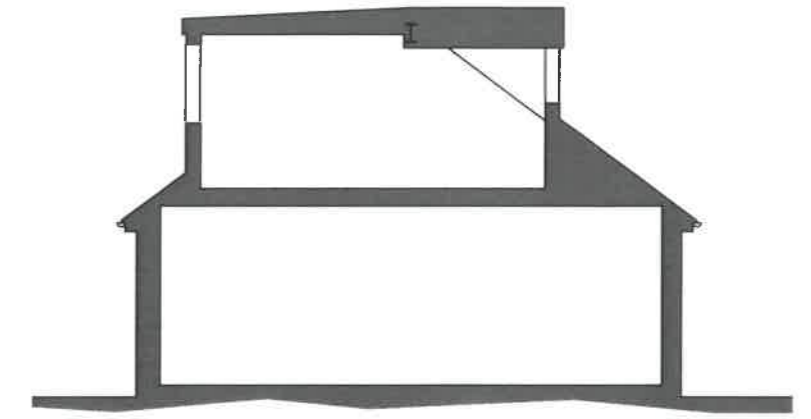
Typical Section B
