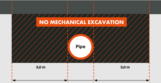
Figure 1. Excavation restrictions
