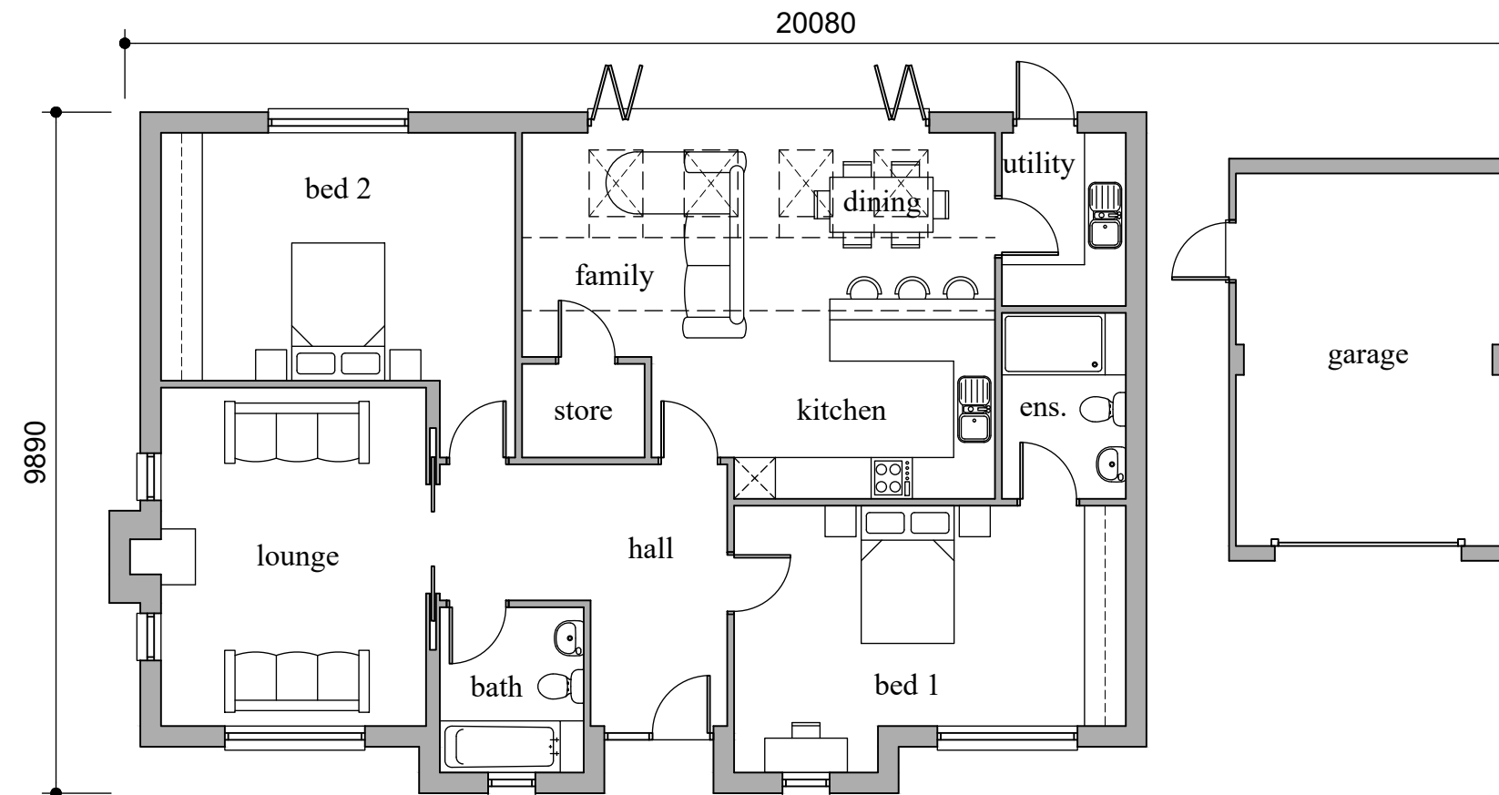
Floor Plan 123.6 sqm
