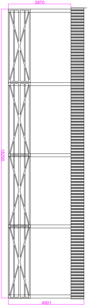
Proposed South Elevation 1:50
