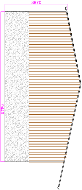
Proposed West Elevation 1:50
