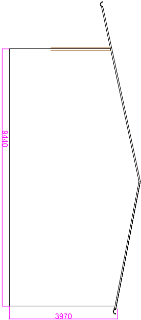
Proposed East Elevation 1:50
