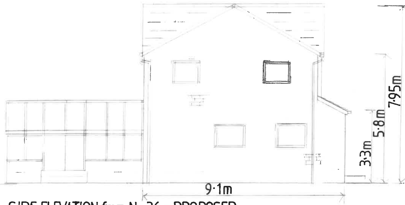
SIDE ELEVATION from No 36 - PROPOSED
