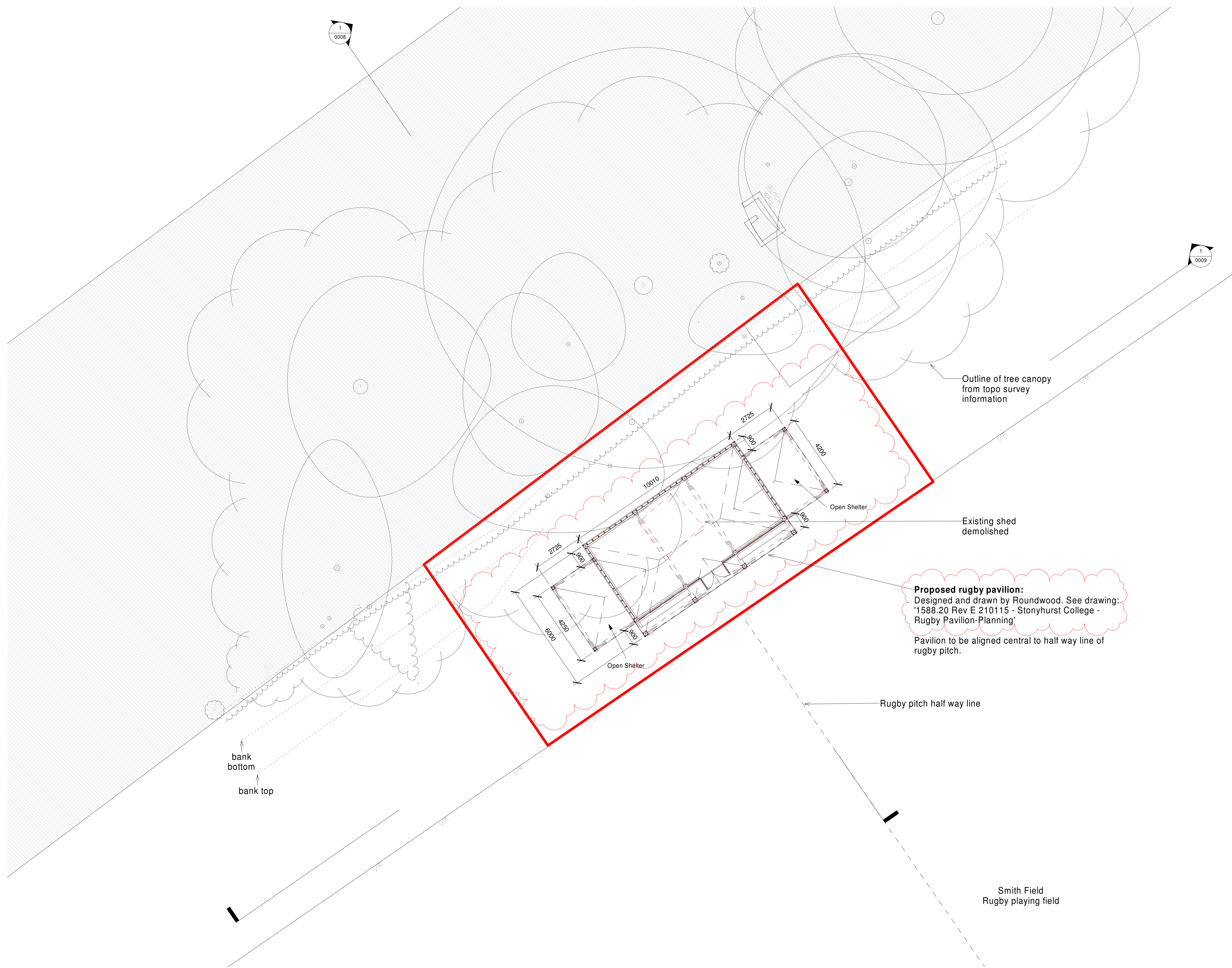
1 Proposed Block Plan 1 : 100
