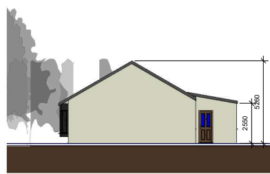
⑤ Existing North-East Elevation 1:100
