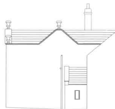
Existing North Elevation inside the courtyard showing extg s&vp connection
