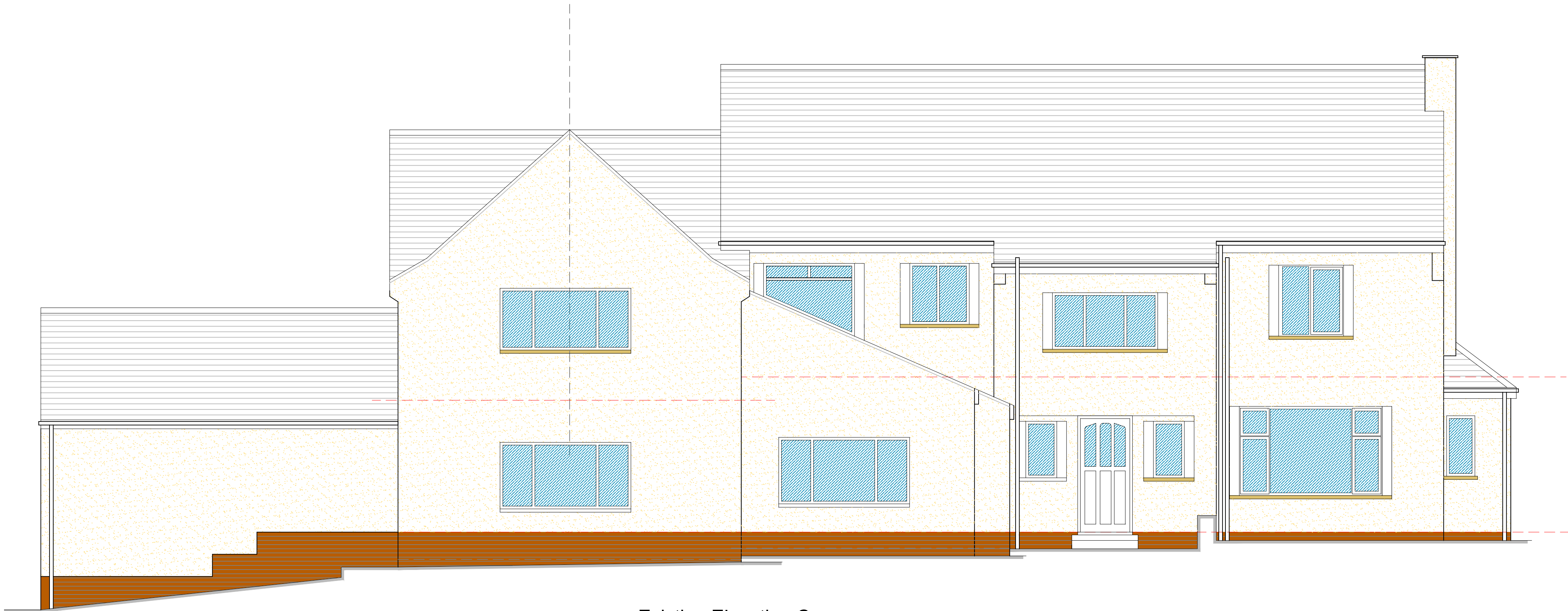
Existing Elevation C - Scale 1:50 (REAR)
