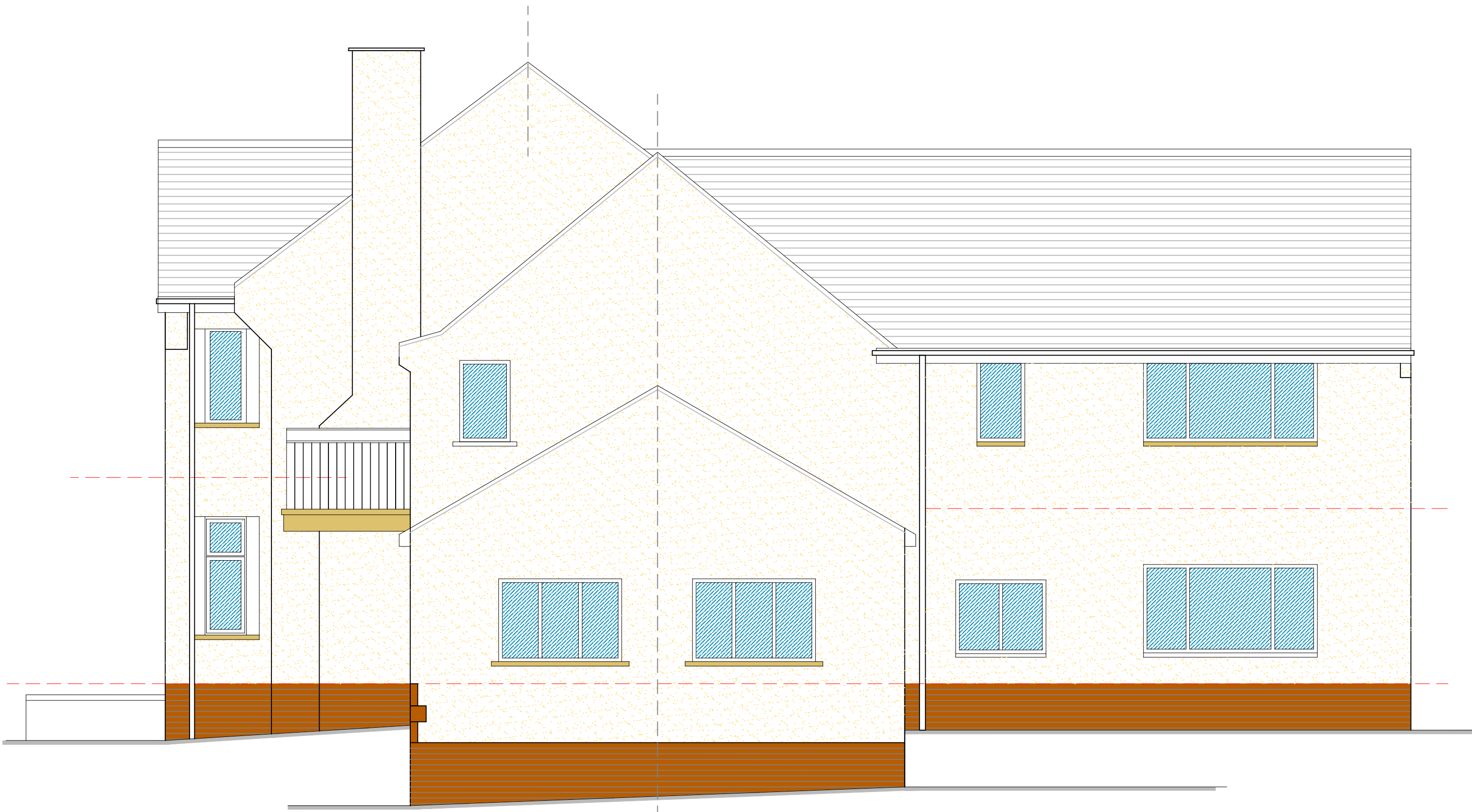
Existing Elevation D - Scale 1:50 (RIGHT)
