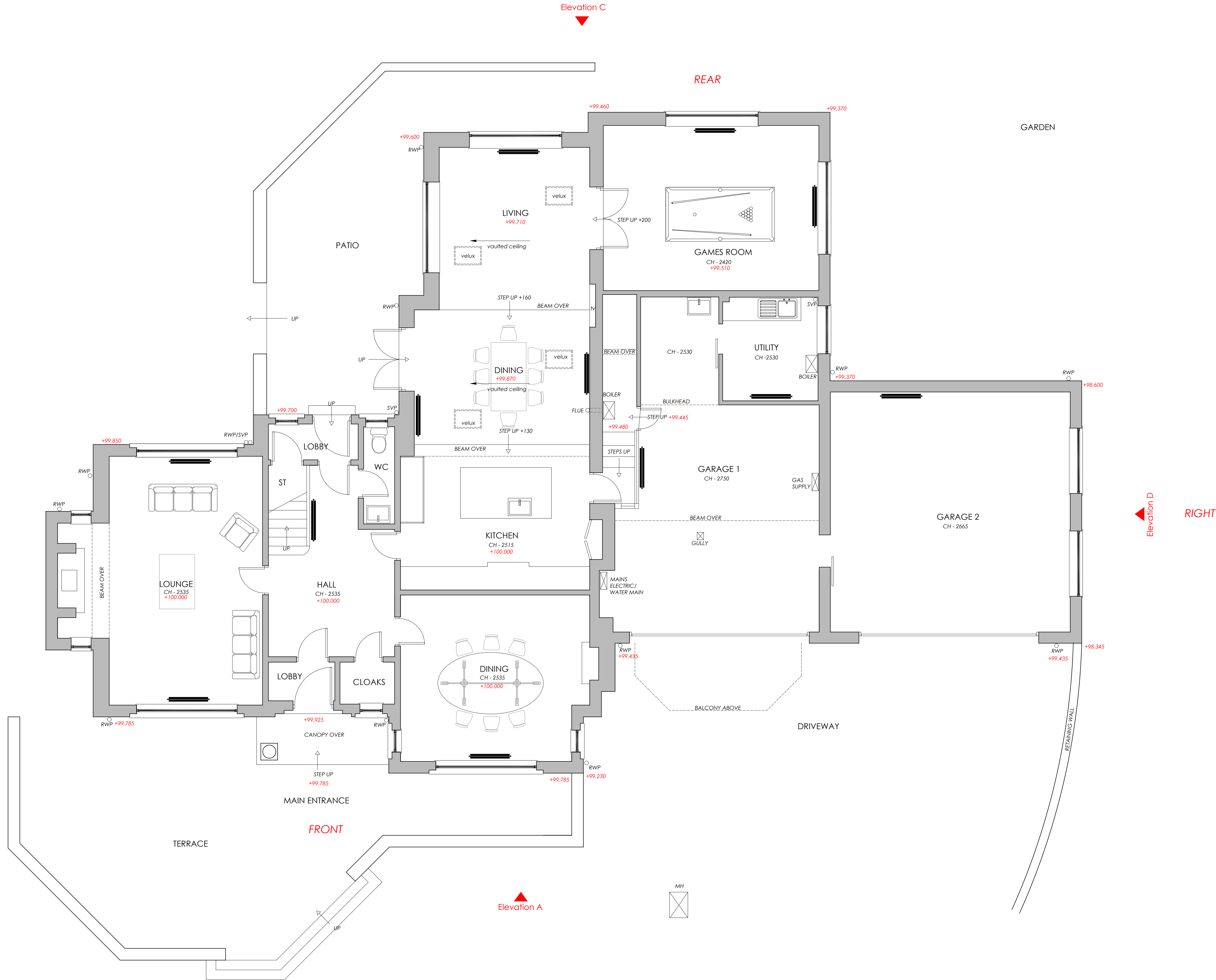
Existing Ground Floor Plan - Scale 1:50
