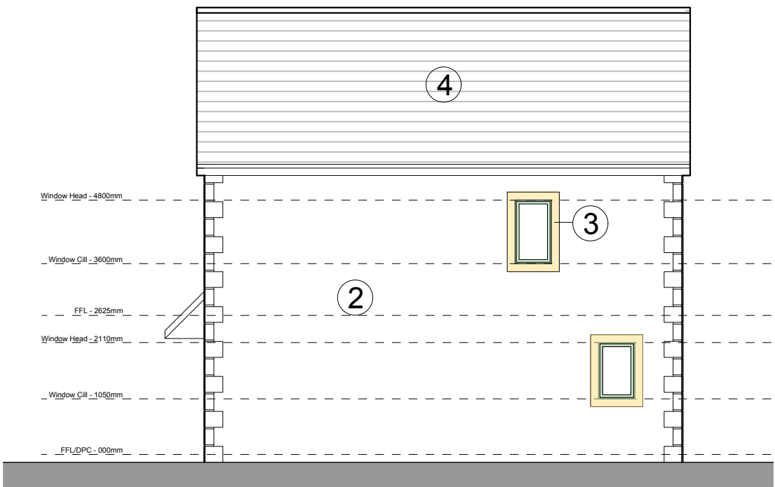
Side Elevation
