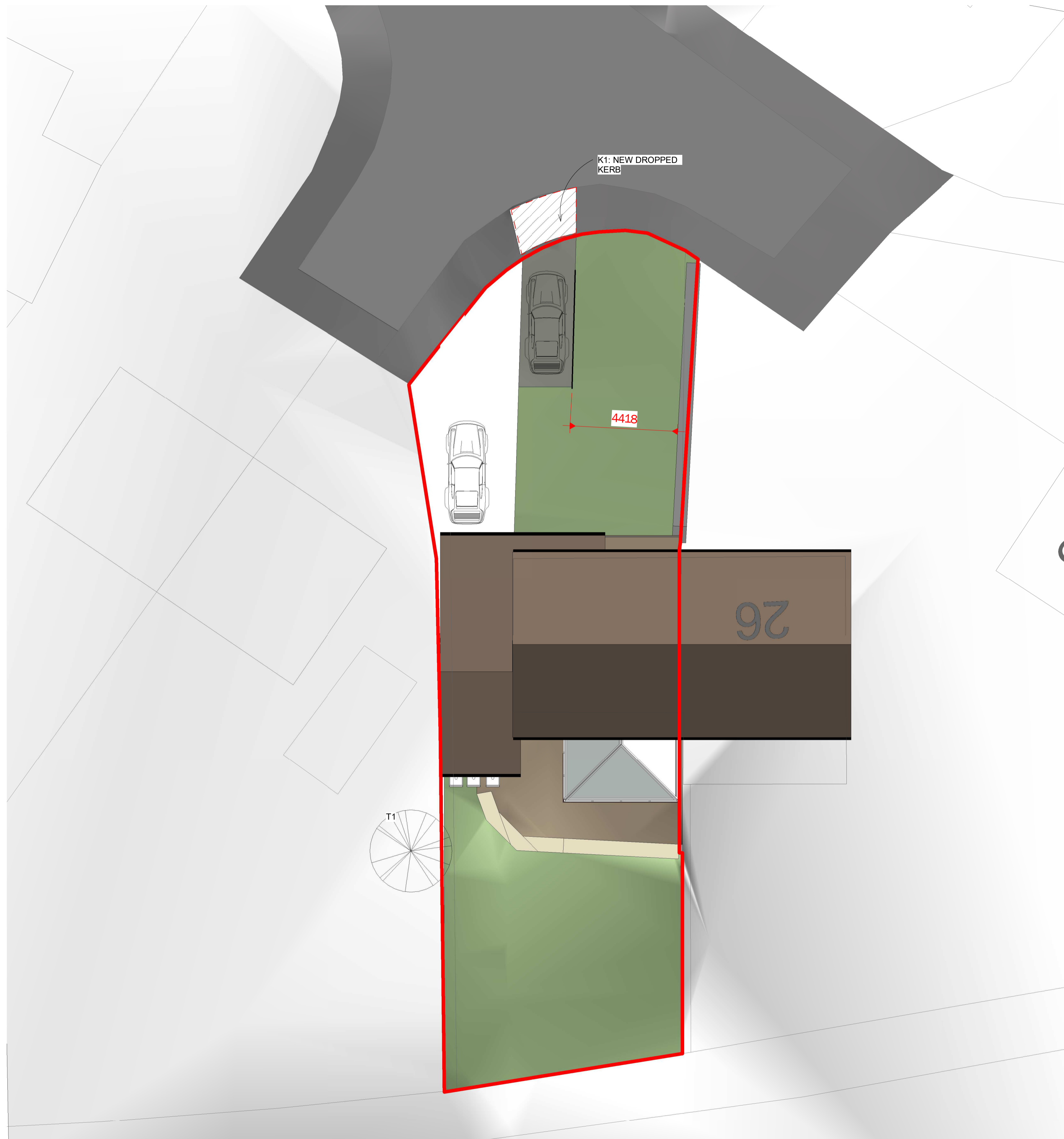
1 PROPOSED SITE PLAN 1 : 100
