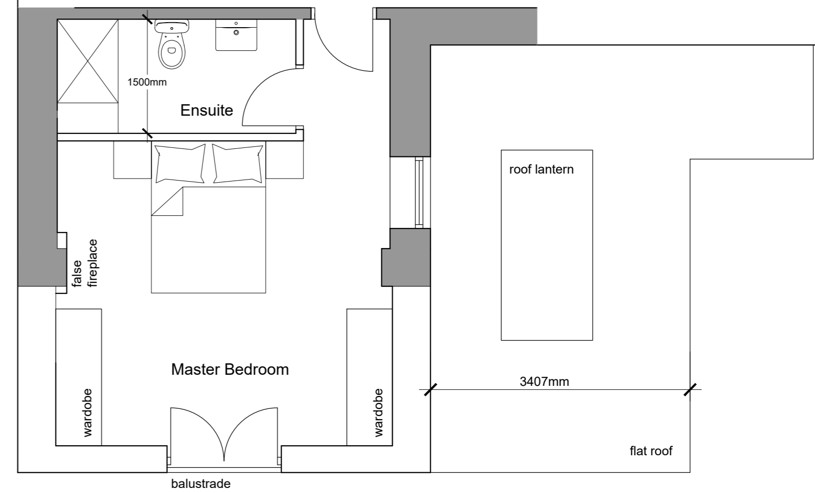
Part First Floor Plan 1:50
