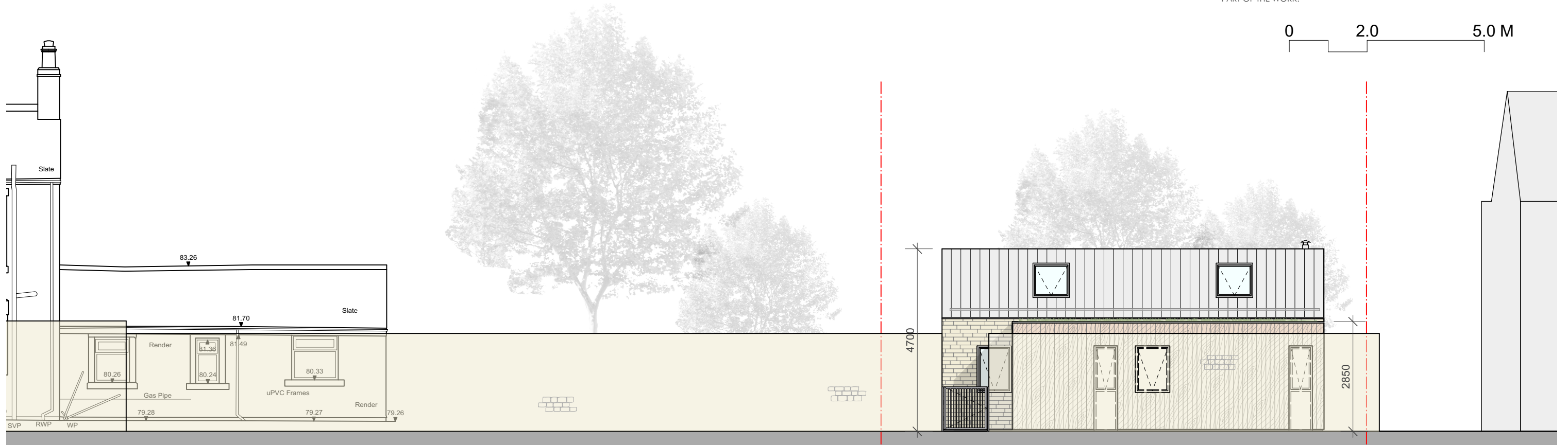
1 PROPOSED SOUTH EAST ELEVATION Scale: 1:100
