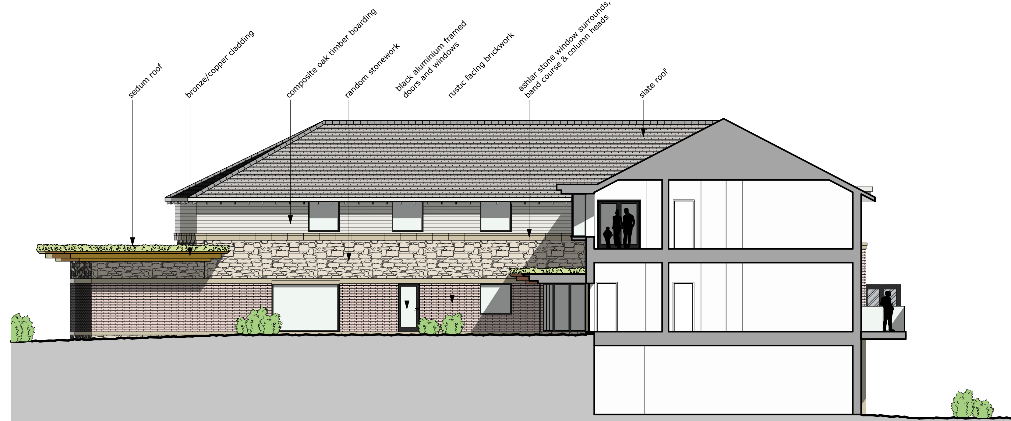
south west elevation
