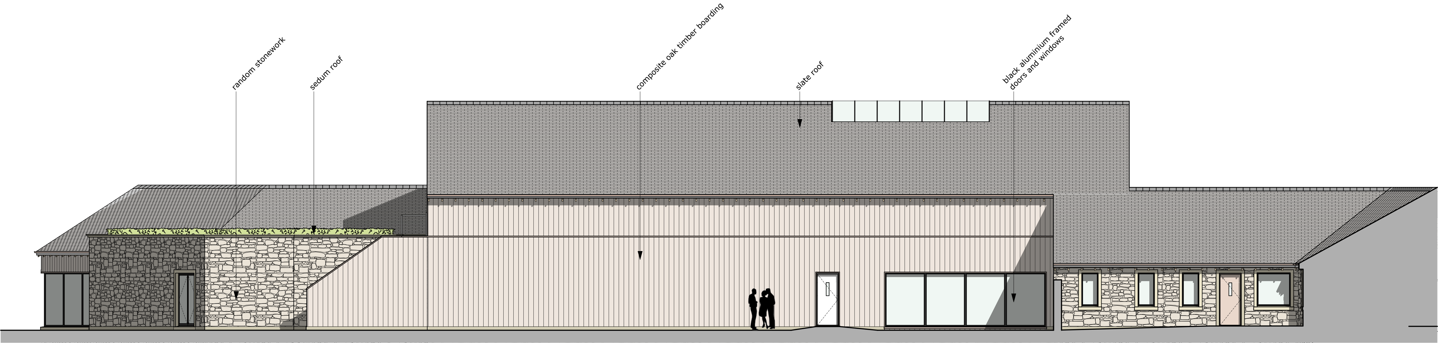
proposed south west elevation (8)
