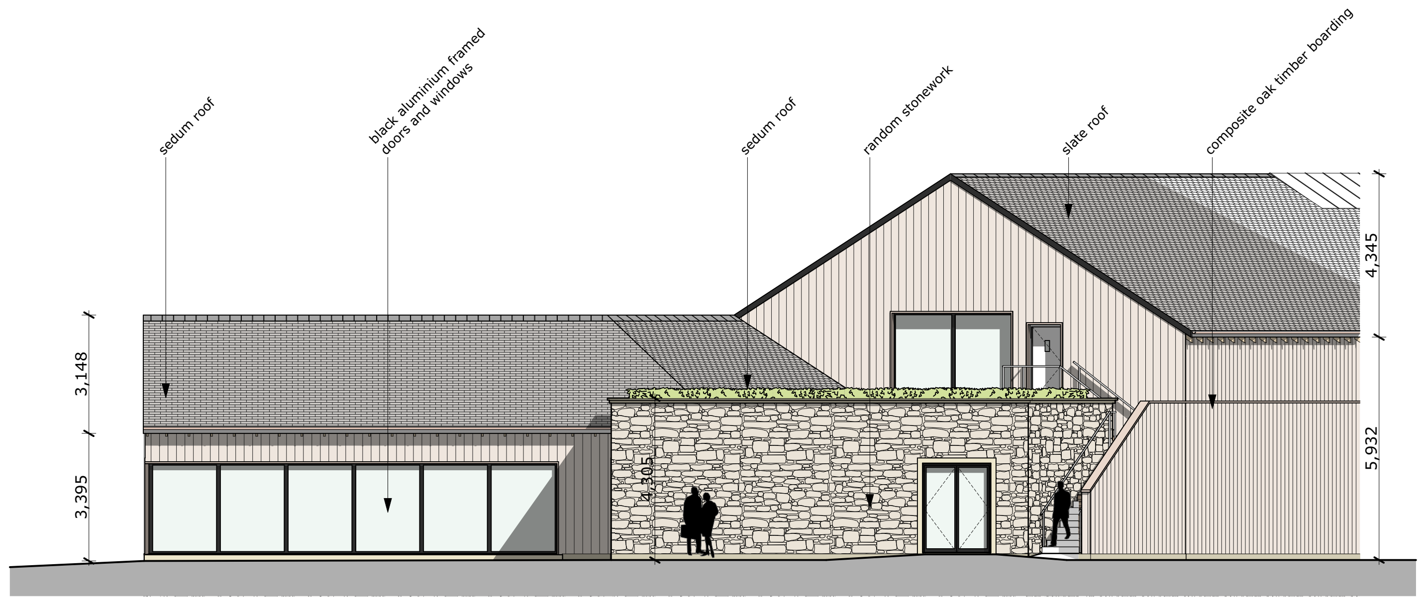
proposed south west elevation (7)
