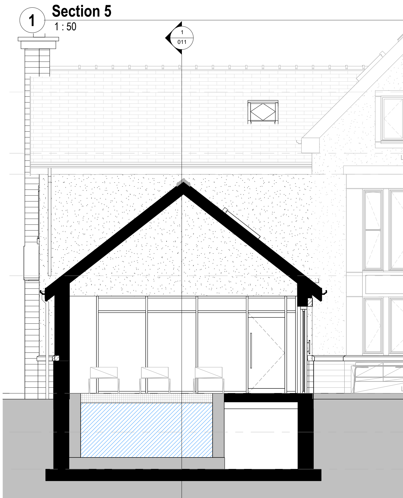
2 GA Section - Gymnasium Copy 1 1:50
