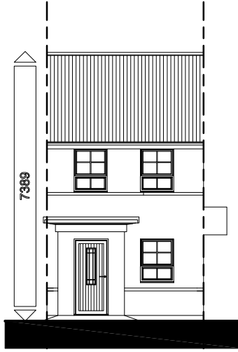
FRONT ELEVATION
