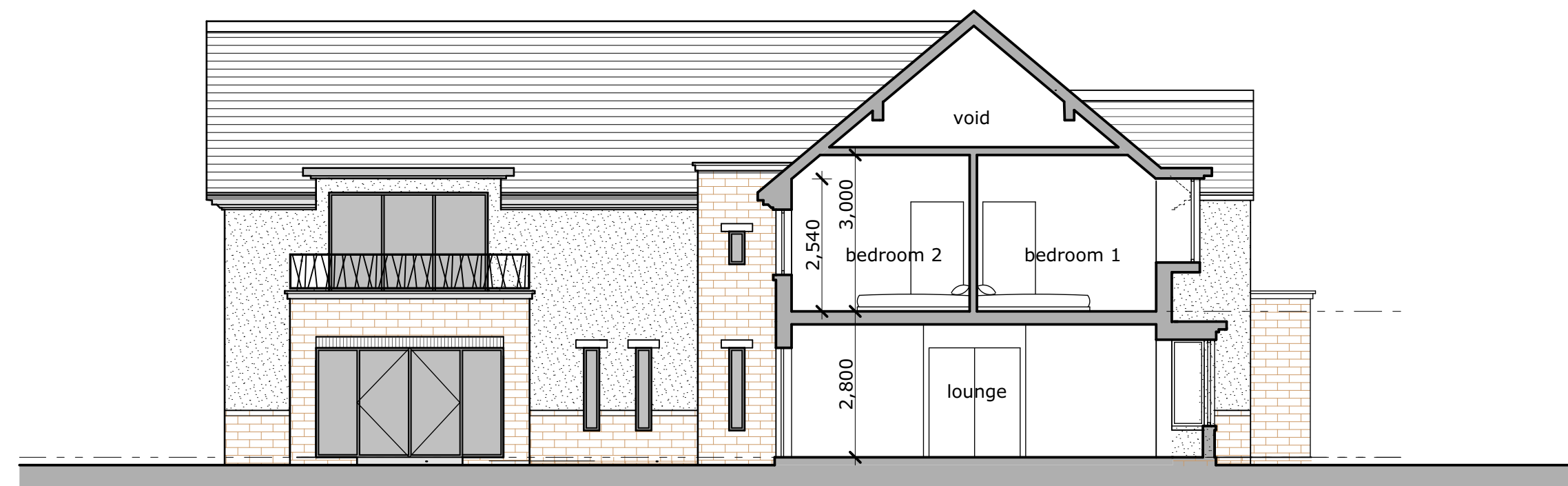
section B-B
