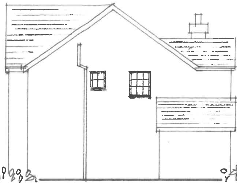
Side Elevation to No. 30
