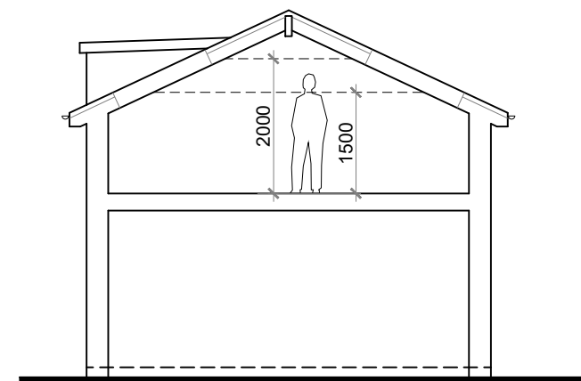
SECTIONAL VIEW
