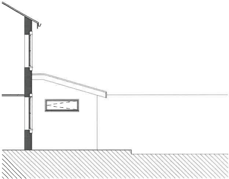
4 EXISTING NO. 9 SOUTH 1 : 50
