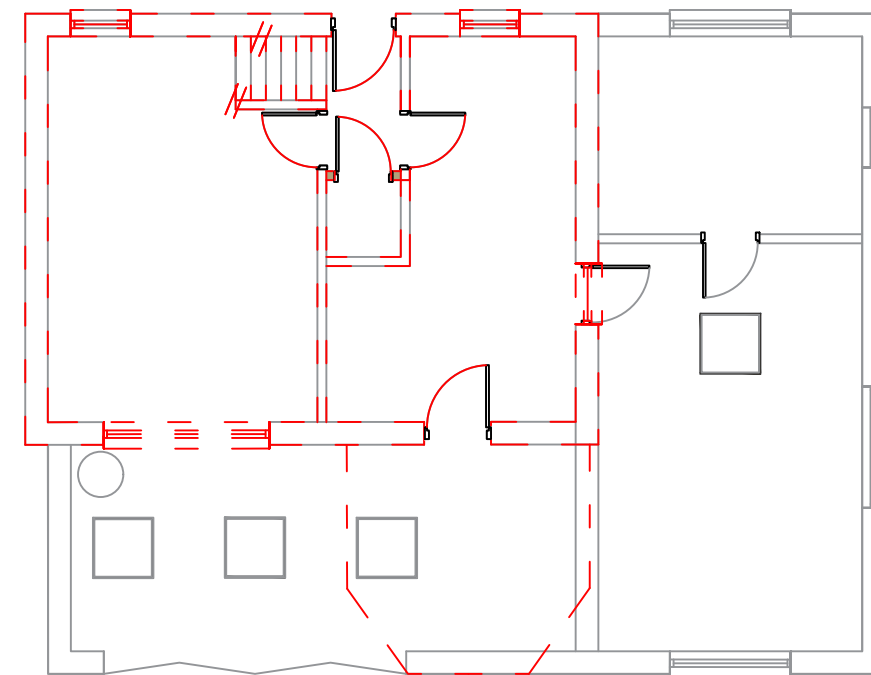
Existing/Proposed Overlay (1:100)
