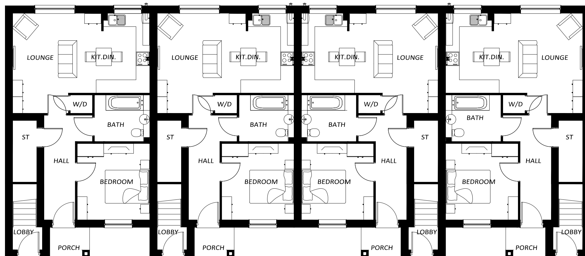
Ground Floor
