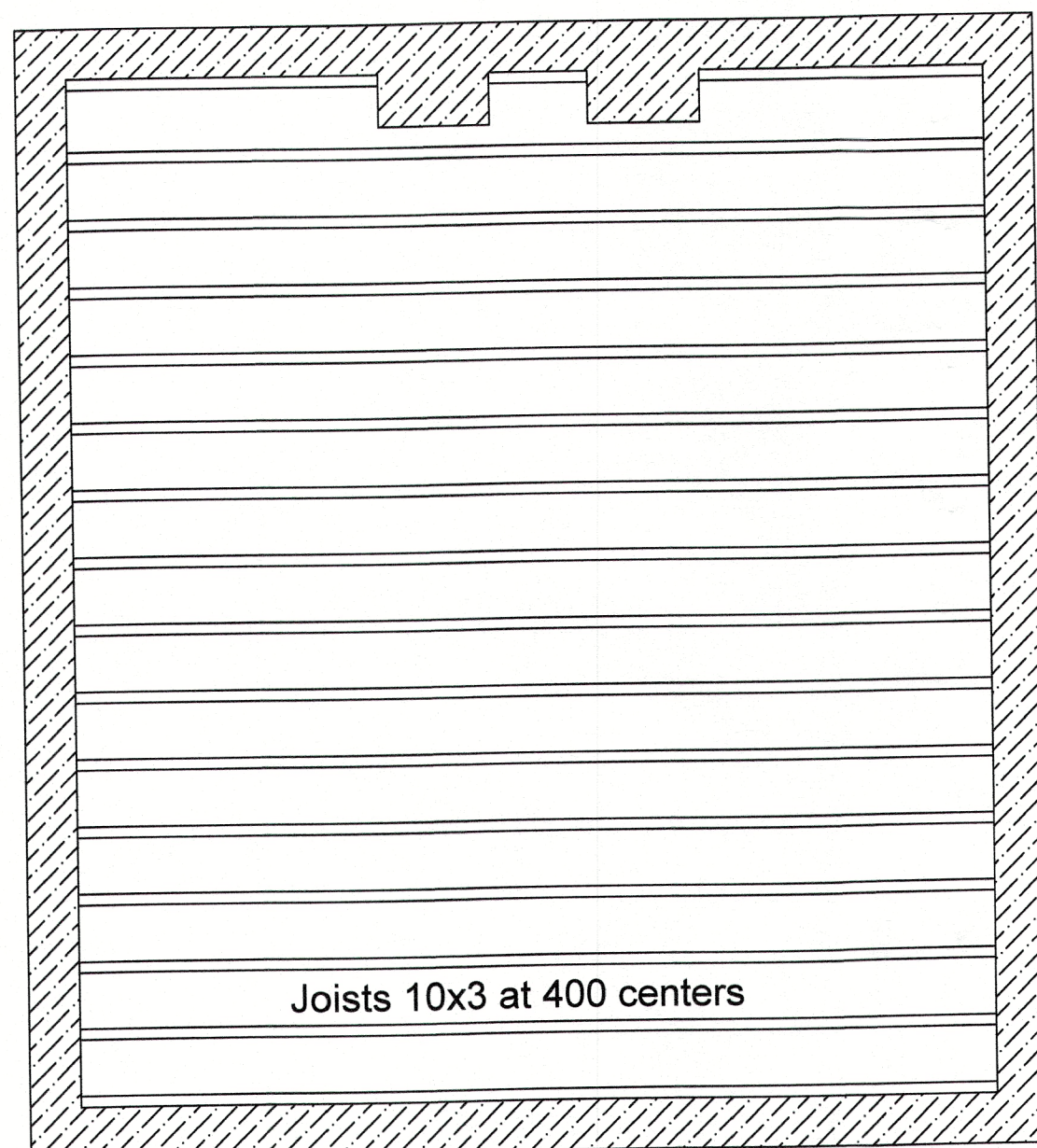
Loft Floor Plan Existing
