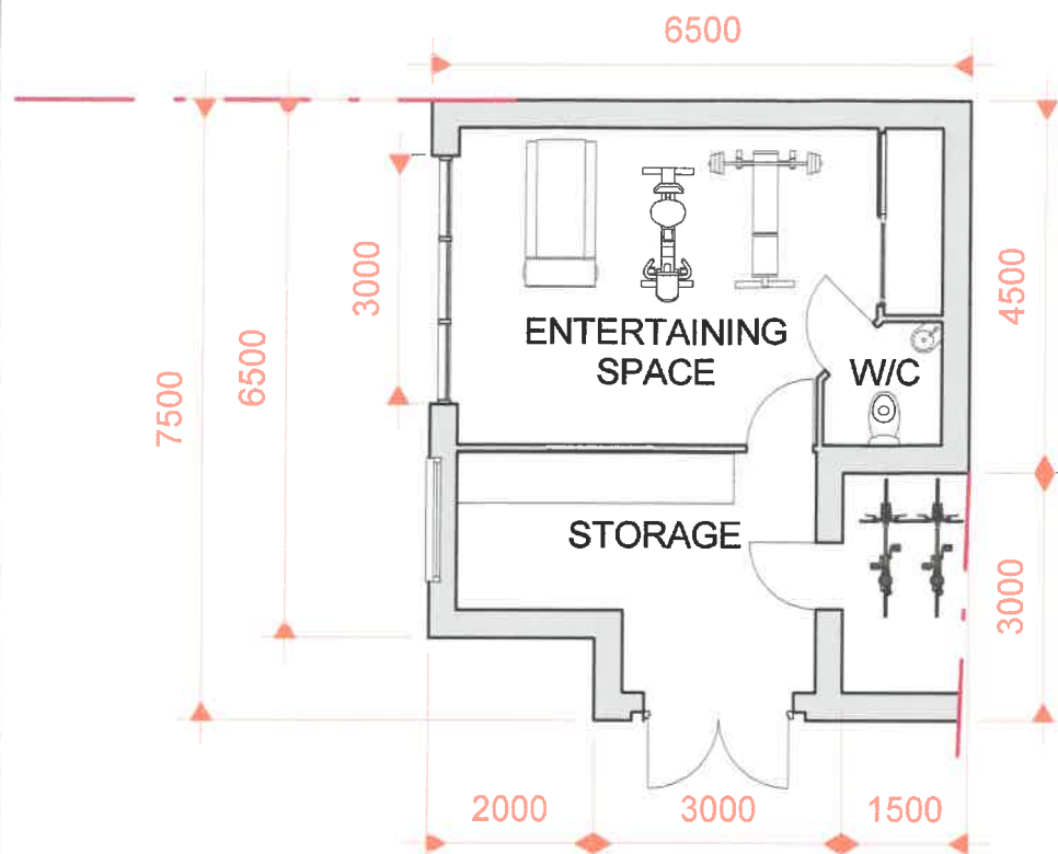
0 PROPOSED GROUND FLOOR
