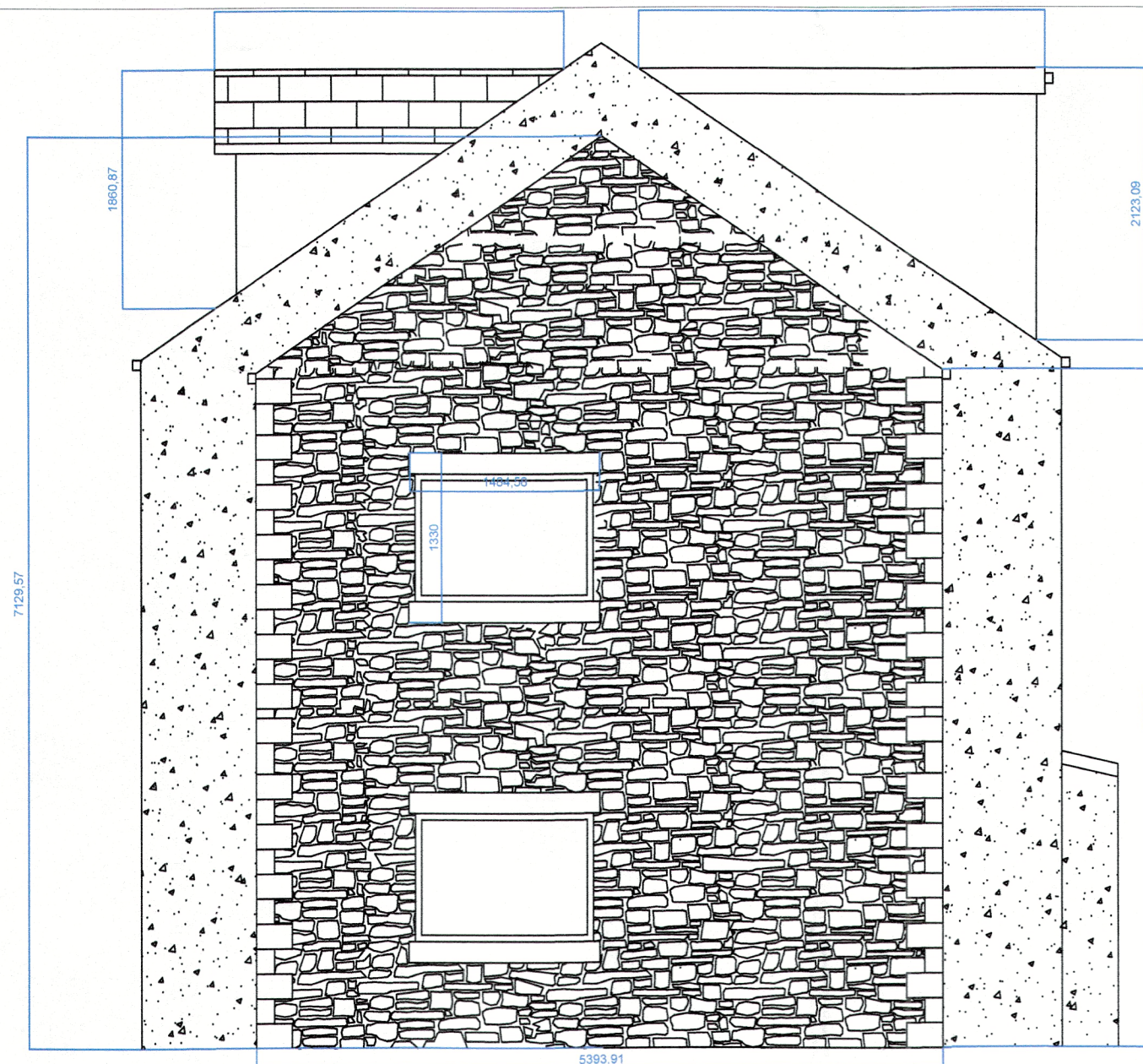
Side Elevation Proposed
