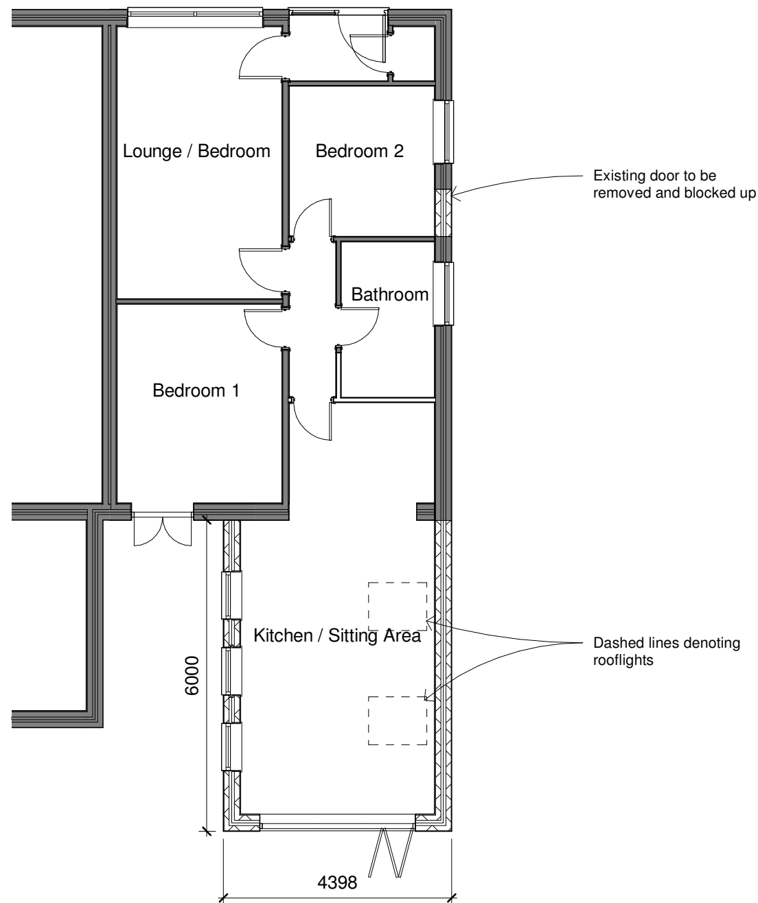
Proposed Ground floor 1 : 100
