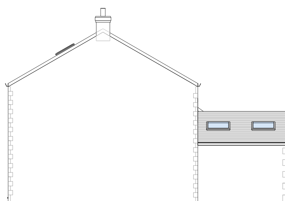
Proposed Side Elevation B (View from No.4) 1 : 100
