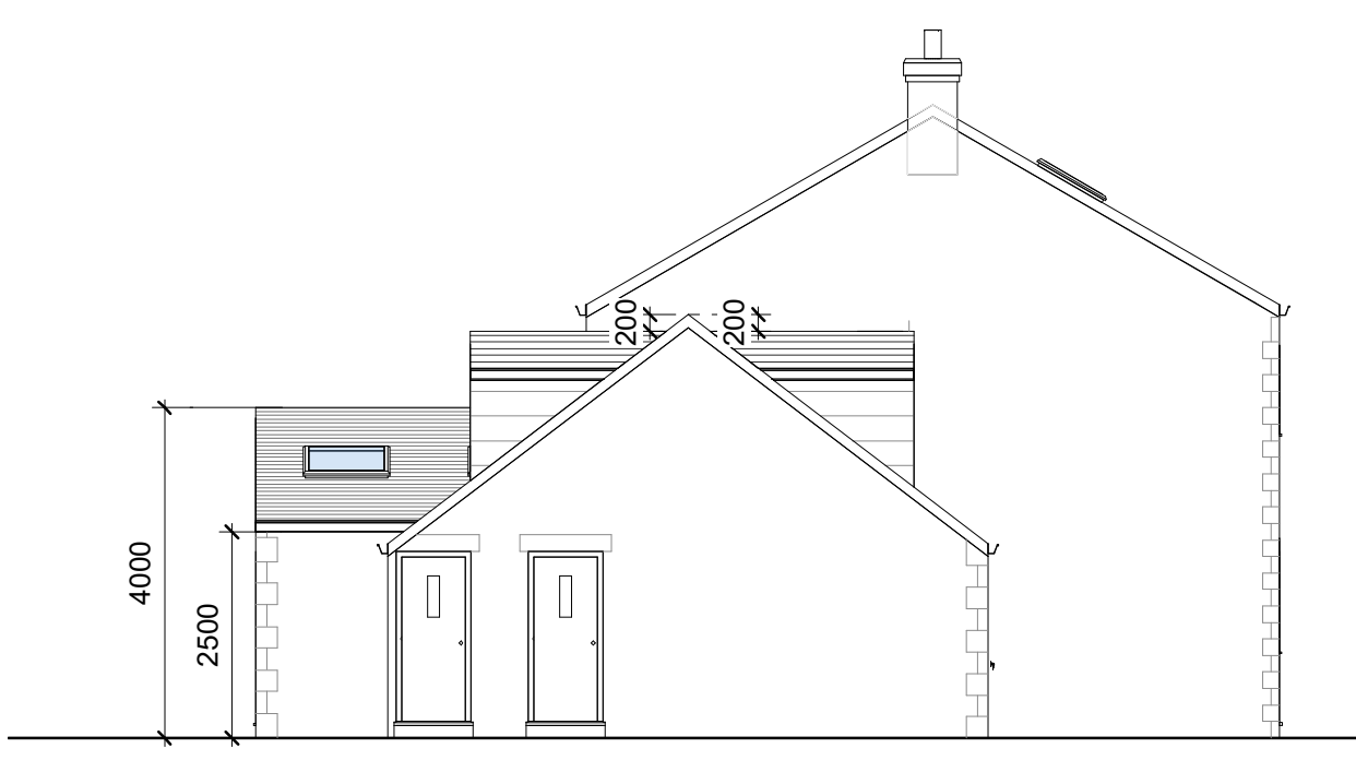
Proposed Side Elevation A (View from No.17) 1 : 100
