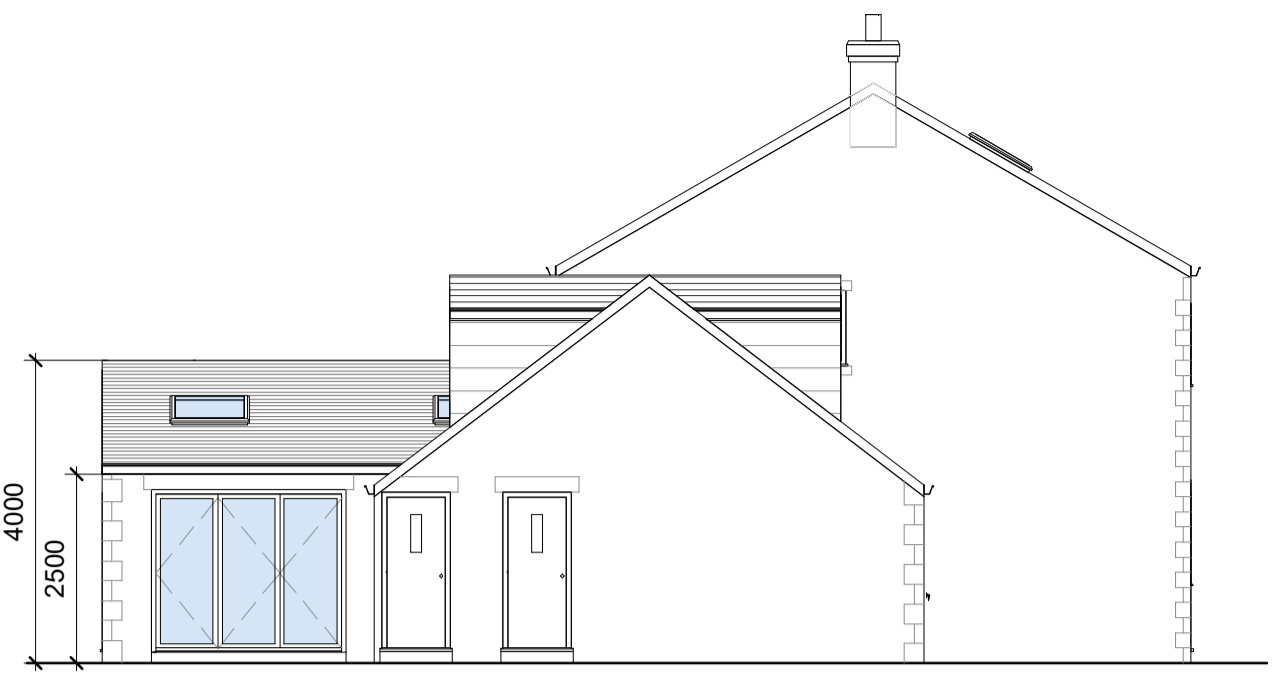
Proposed Side Elevation A (View from No.17) 1 : 100
