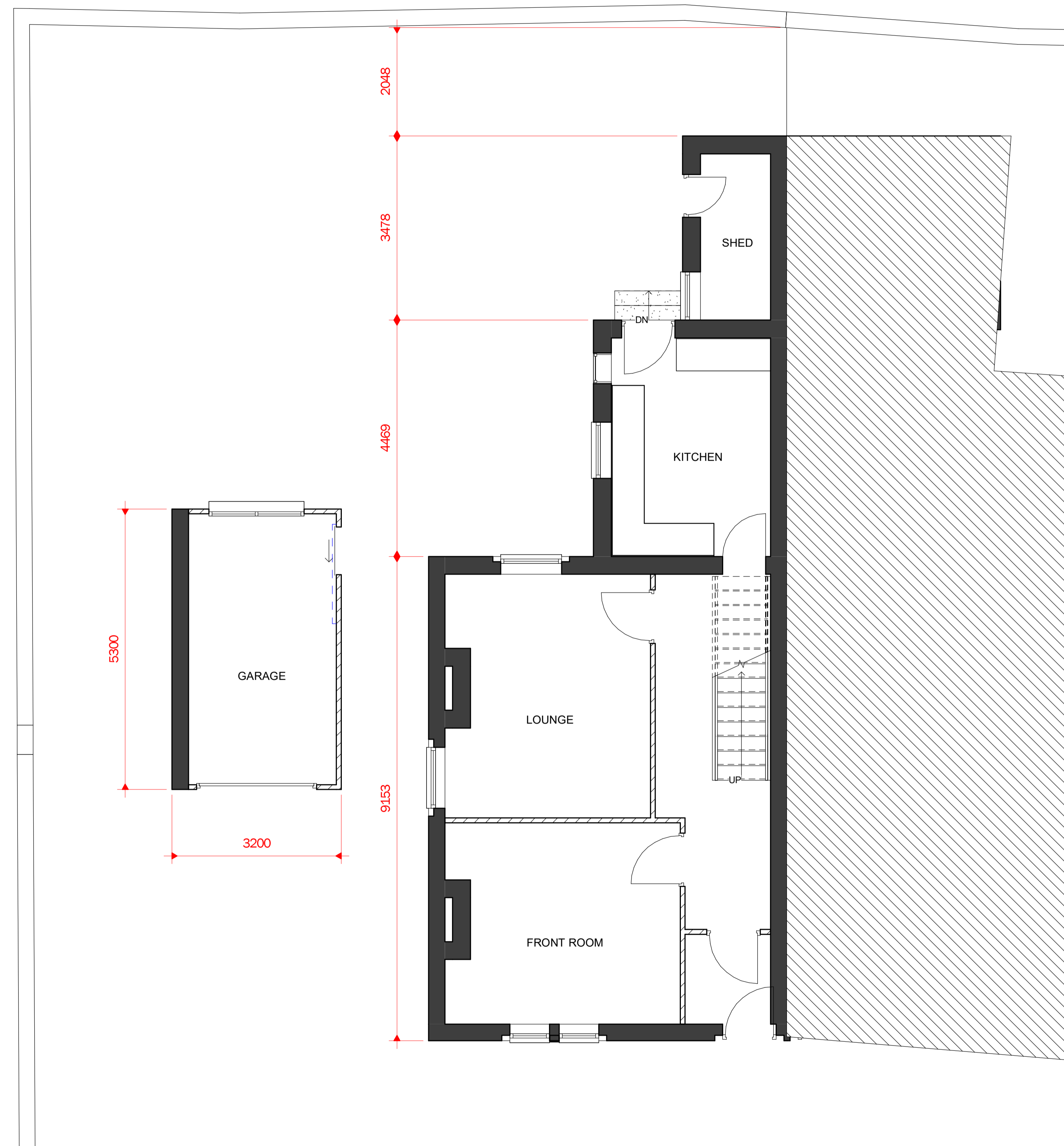
1 0 GROUND FLOOR 1 : 50
