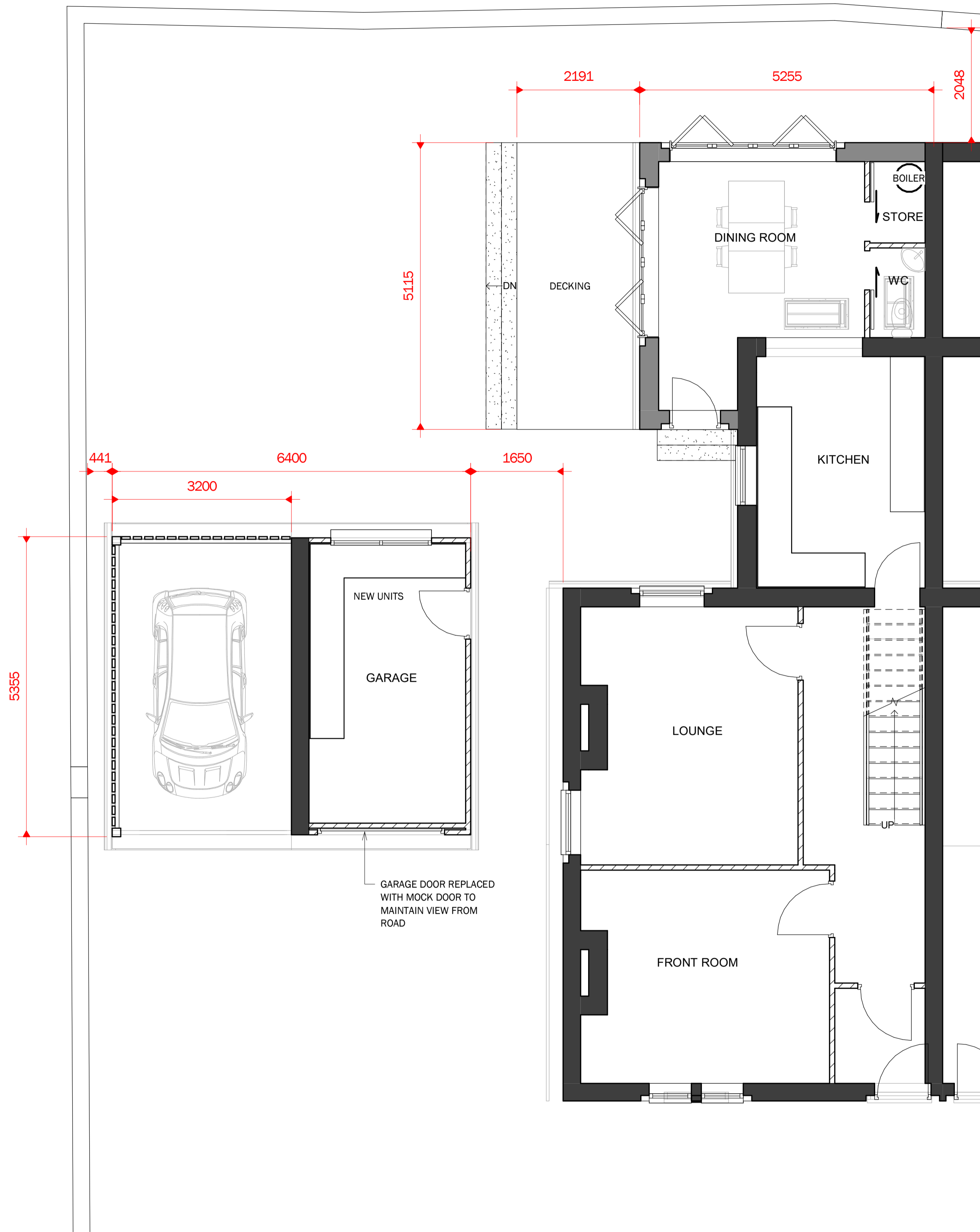
1 0 PROPOSED GROUND FLOOR 1 : 50
